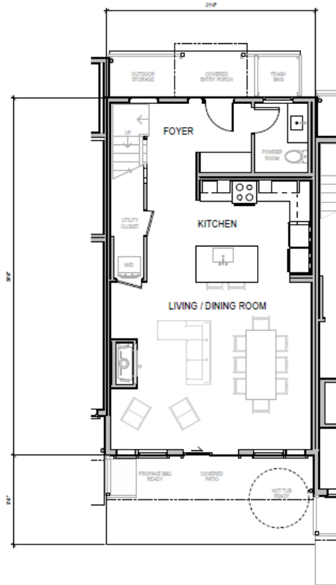
① LEVEL 1 FLOOR PLAN 756 SF
