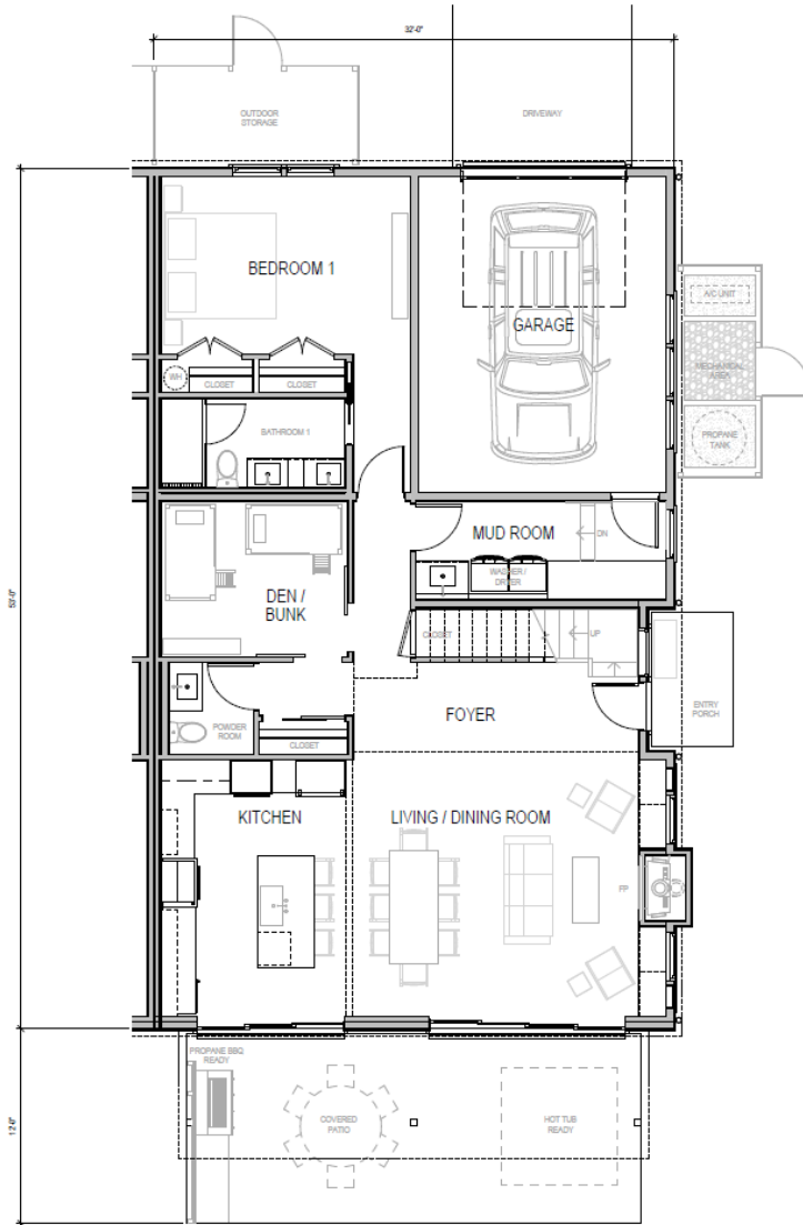
① LEVEL 1 FLOOR PLAN 1,371 SF (+315 SF GARAGE)
