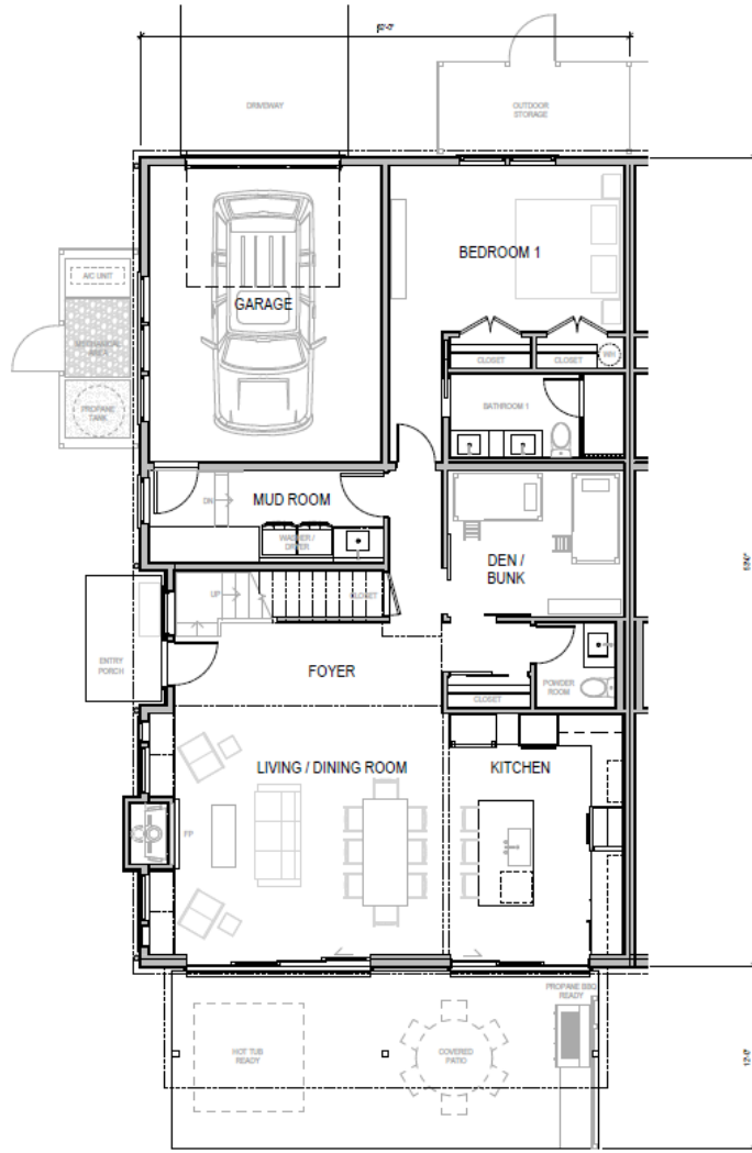
① LEVEL 1 FLOOR PLAN 1,371 SF (+315 SF GARAGE) TOTAL AREA: 2,461 SF
