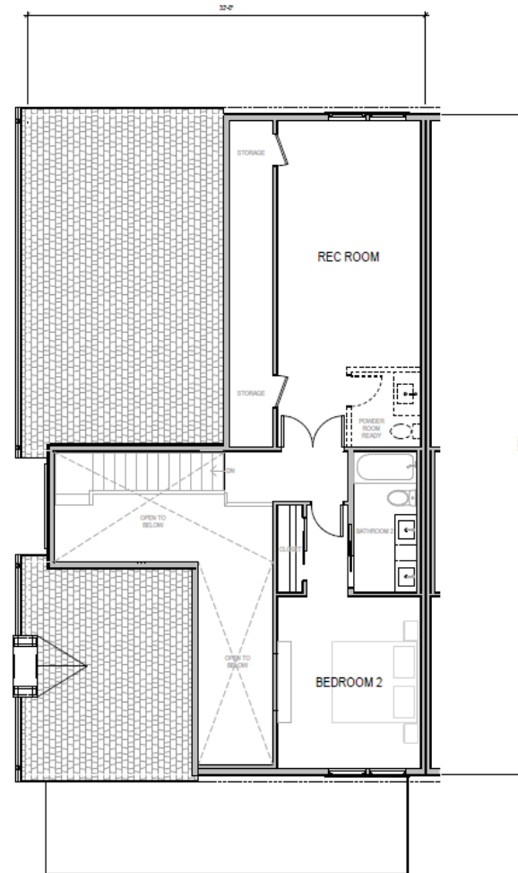
② LEVEL 2 FLOOR PLAN 775 SF
