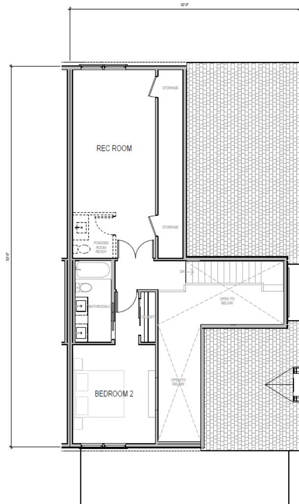
② LEVEL 2 FLOOR PLAN 775 SF
