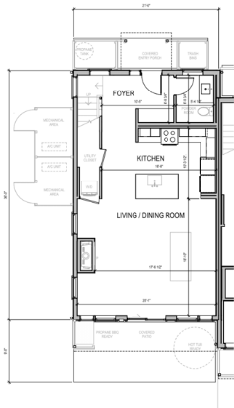
① LEVEL 1 FLOOR PLAN 756 SF SCALE: 1/4" = 1'-0"
