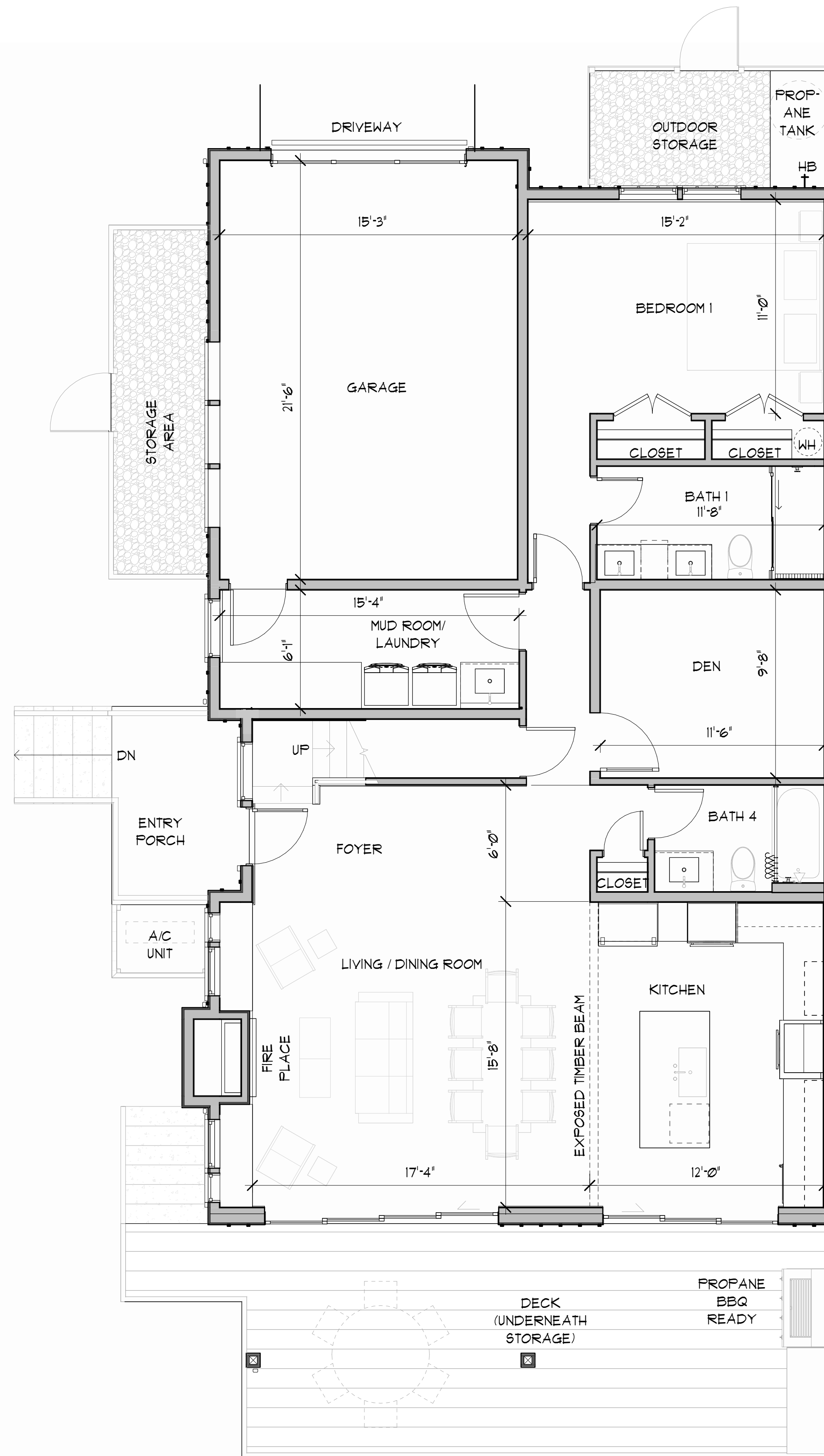
LEVEL 1 FLOOR PLAN
