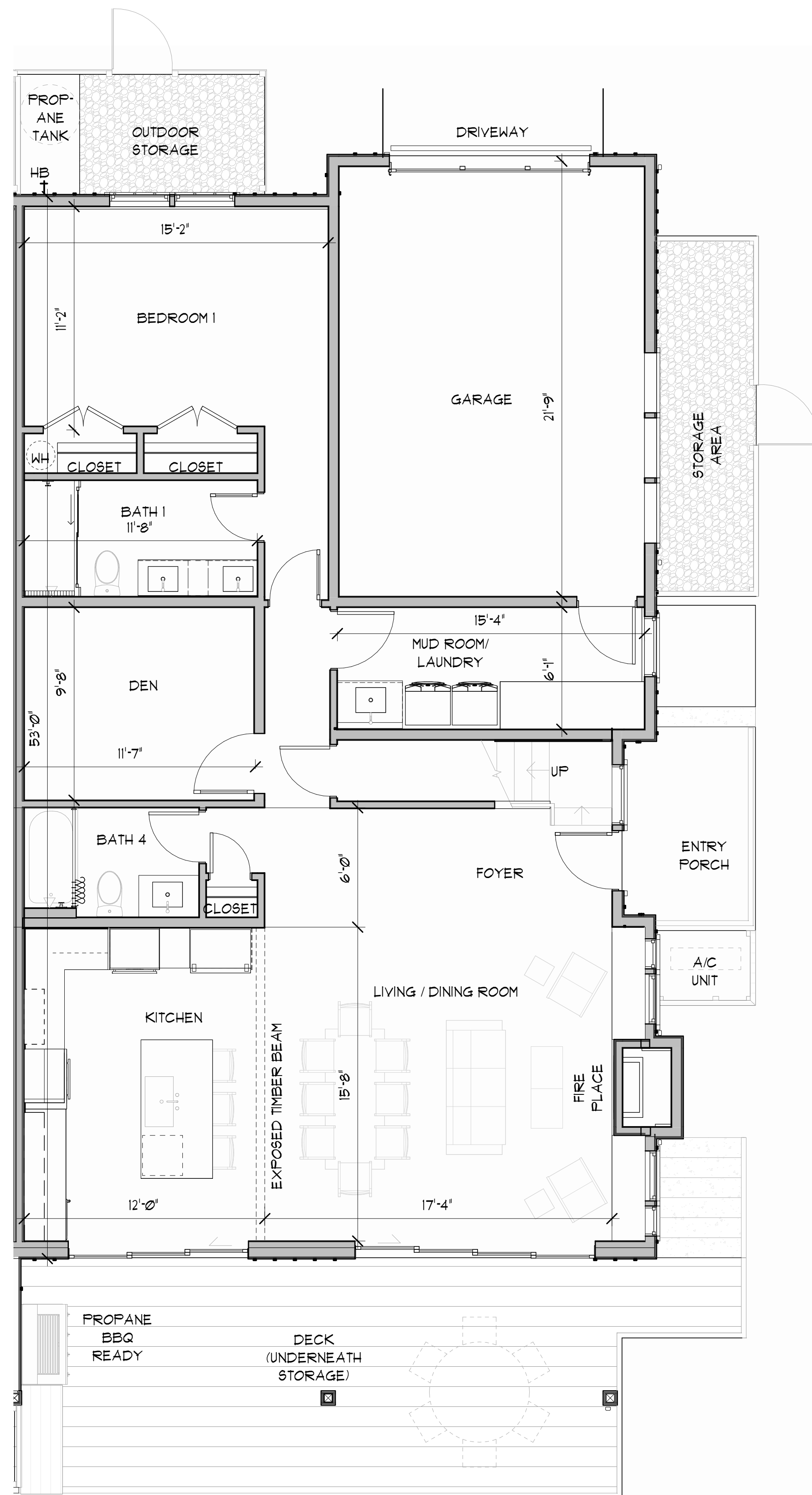
LEVEL 1 FLOOR PLAN
